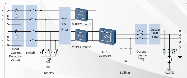
SUN2000-8/12KTL
